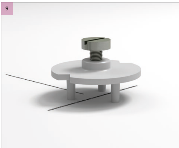
Insert the distance holders into the backside of the wall panel. See 9 - Result.
